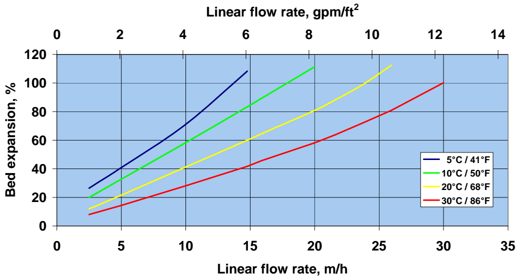
Figure 19 Backwash expansion
